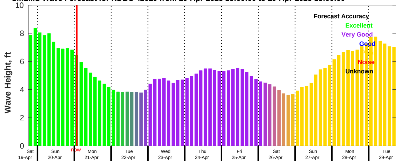
CMEMS Wave Forecast for NDBC 42019 from 19-Apr-2025 18:00:00 to 29-Apr-2025 18:00:00
