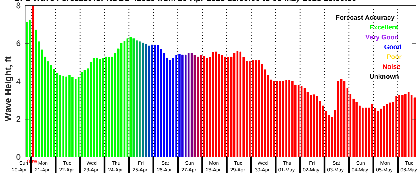
GFS Wave Forecast for NDBC 42019 from 20-Apr-2025 18:00:00 to 06-May-2025 18:00:00
