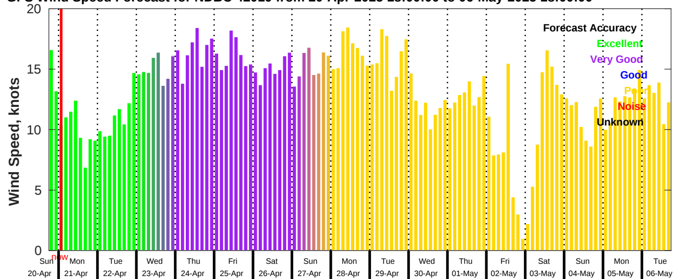
GFS Wind Speed Forecast for NDBC 42019 from 20-Apr-2025 18:00:00 to 06-May-2025 18:00:00
