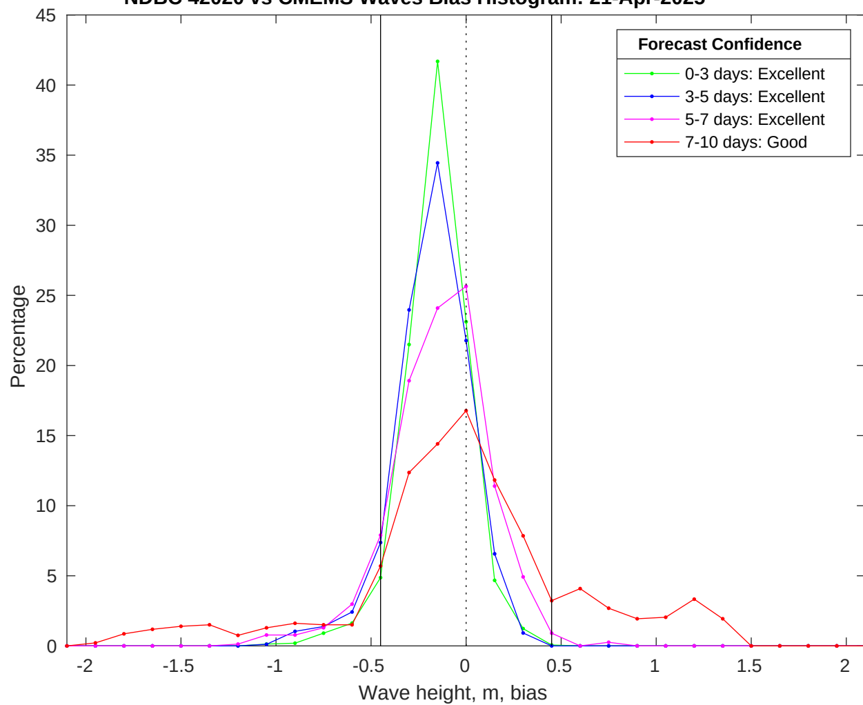
NDBC 42020 vs CMEMS Waves Bias Histogram: 21-Apr-2025
