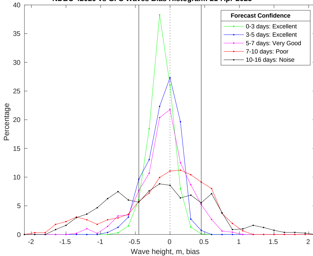
NDBC 42020 vs GFS Waves Bias Histogram: 21-Apr-2025
