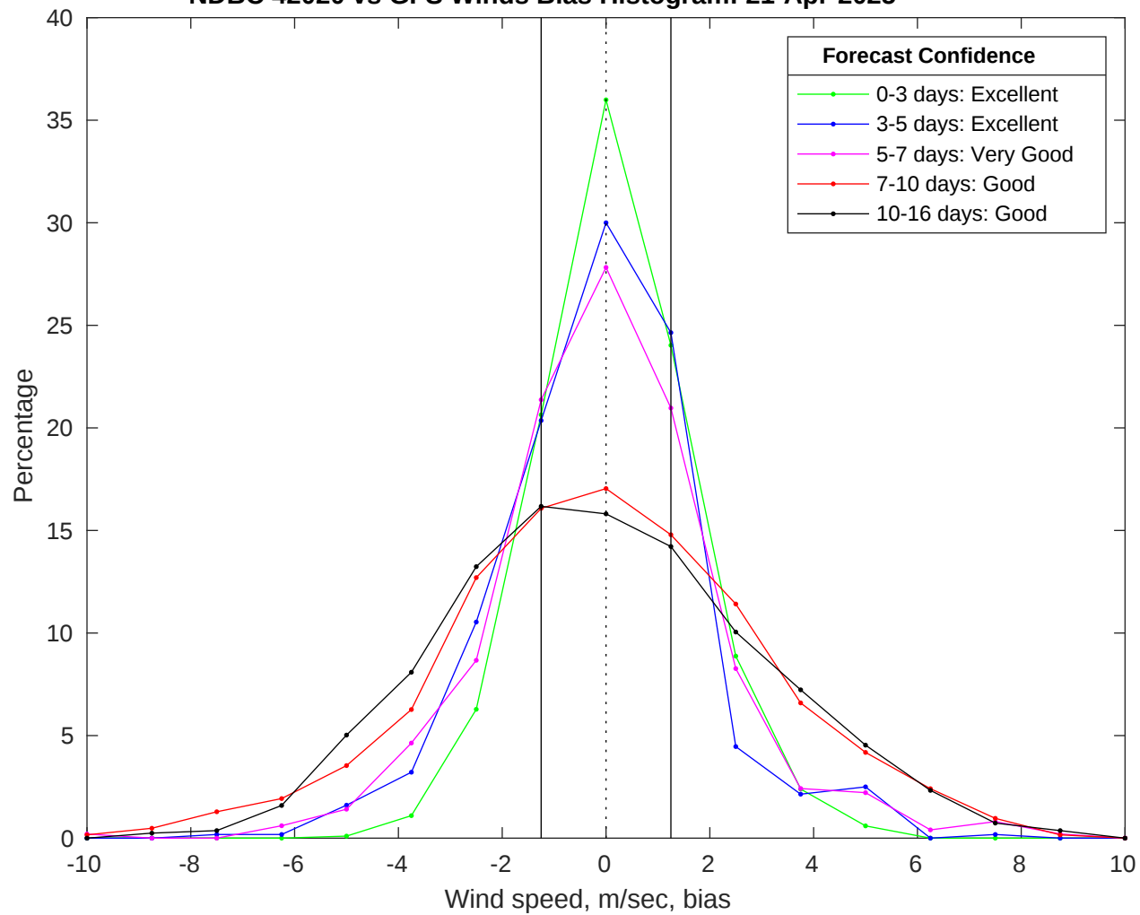
NDBC 42020 vs GFS Winds Bias Histogram: 21-Apr-2025
