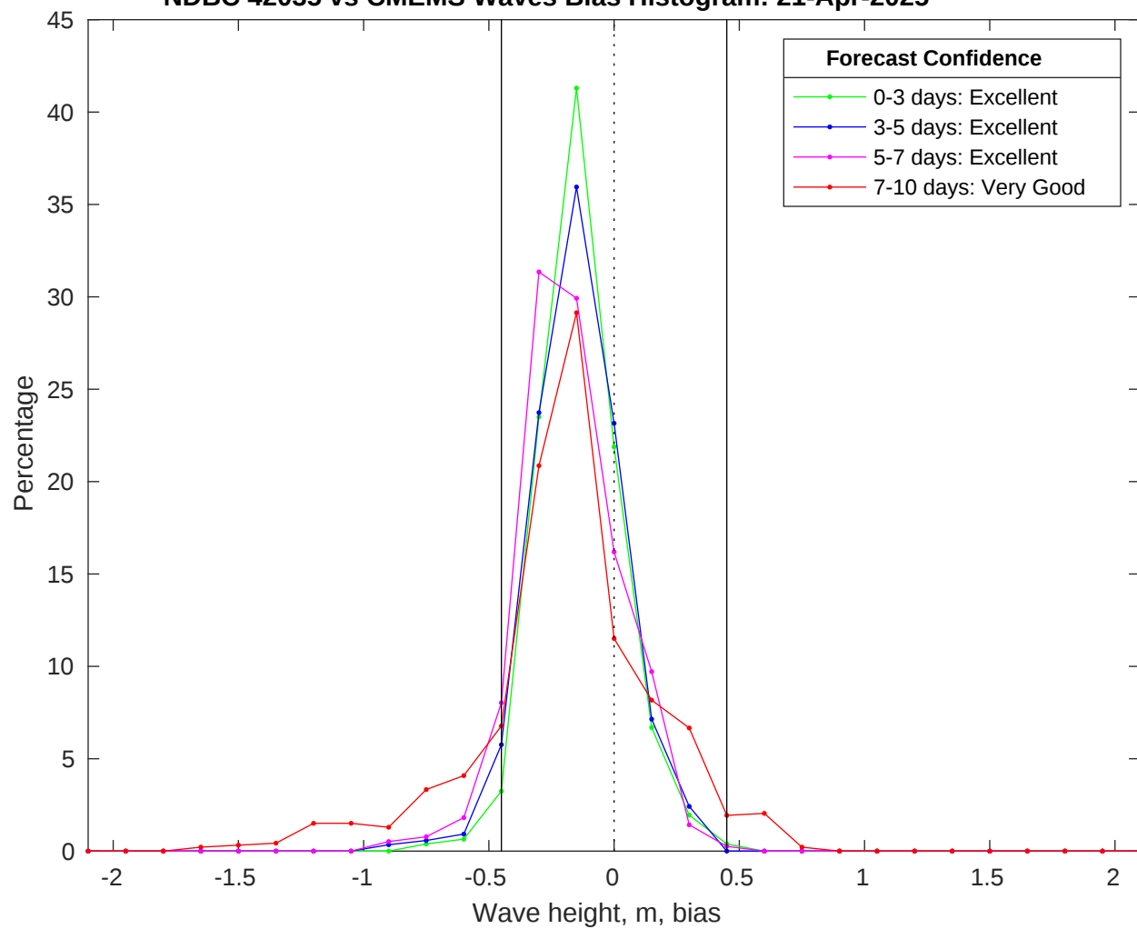
NDBC 42035 vs CMEMS Waves Bias Histogram: 21-Apr-2025
