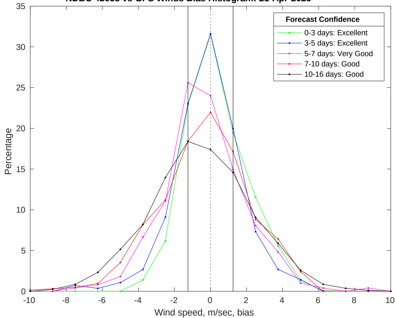
NDBC 42035 vs GFS Winds Bias Histogram: 21-Apr-2025
