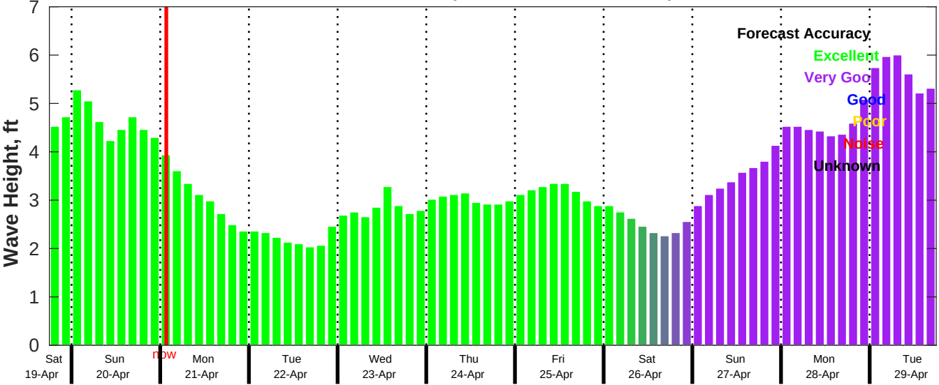
CMEMS Wave Forecast for NDBC 42035 from 19-Apr-2025 18:00:00 to 29-Apr-2025 18:00:00
