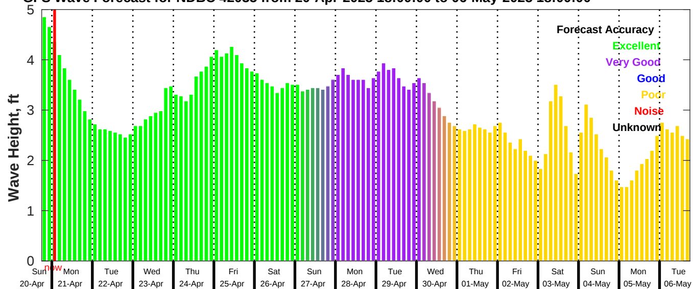
GFS Wave Forecast for NDBC 42035 from 20-Apr-2025 18:00:00 to 06-May-2025 18:00:00
