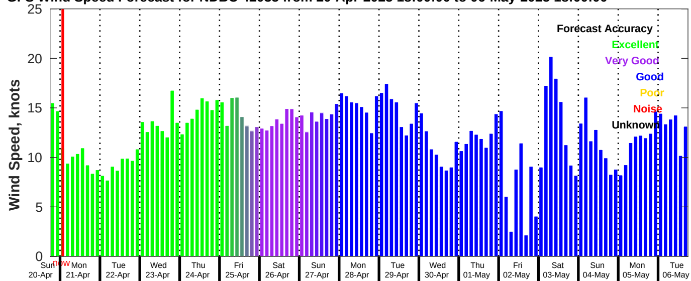
GFS Wind Speed Forecast for NDBC 42035 from 20-Apr-2025 18:00:00 to 06-May-2025 18:00:00
