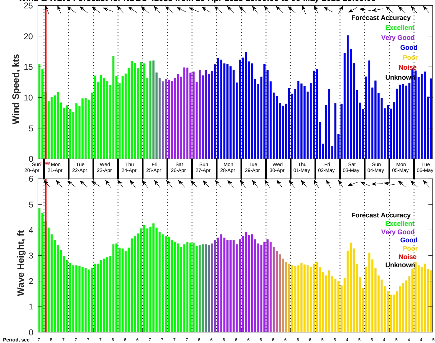
Wind & Wave Forecast for NDBC 42035 from 20-Apr-2025 18:00:00 to 06-May-2025 18:00:00
