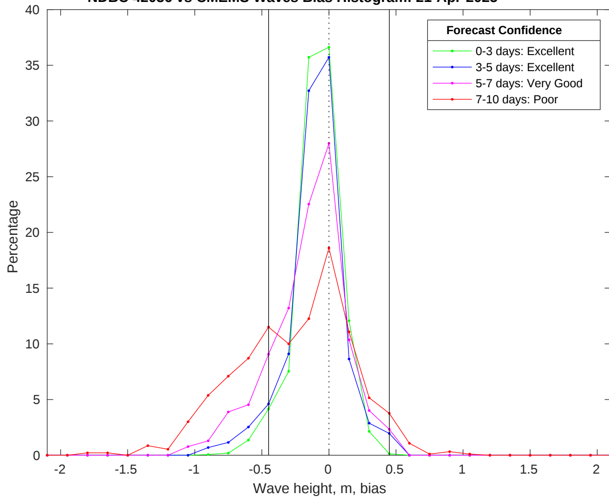
NDBC 42036 vs CMEMS Waves Bias Histogram: 21-Apr-2025
