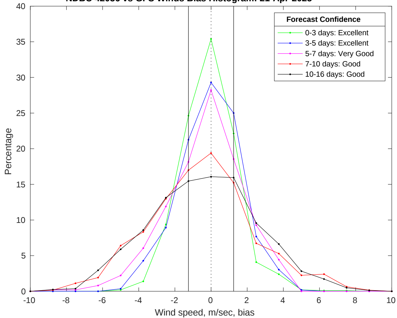
NDBC 42036 vs GFS Winds Bias Histogram: 21-Apr-2025
