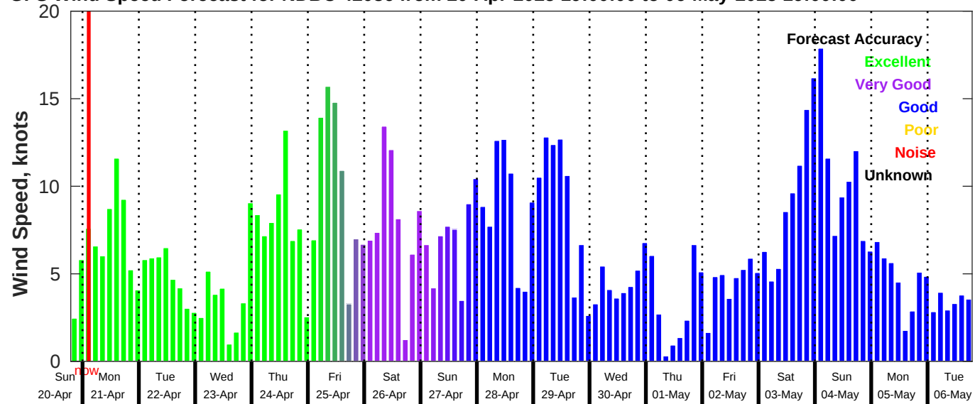
GFS Wind Speed Forecast for NDBC 42036 from 20-Apr-2025 19:00:00 to 06-May-2025 19:00:00
