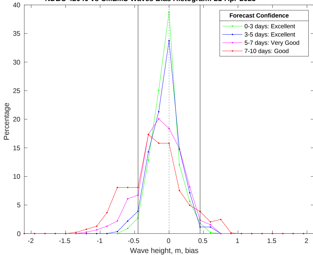
NDBC 42040 vs CMEMS Waves Bias Histogram: 21-Apr-2025
