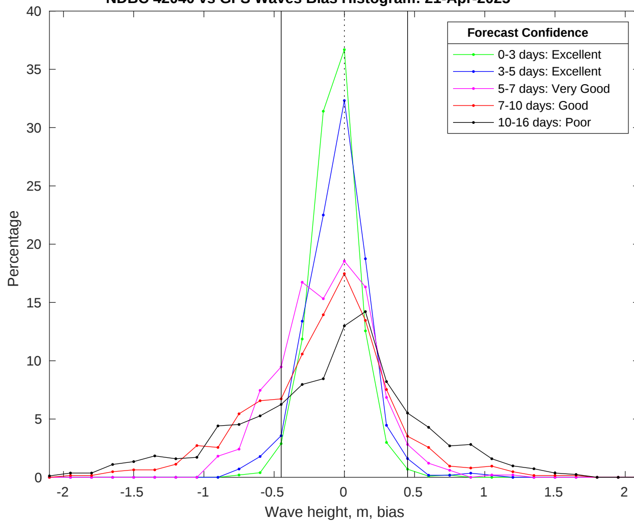
NDBC 42040 vs GFS Waves Bias Histogram: 21-Apr-2025
