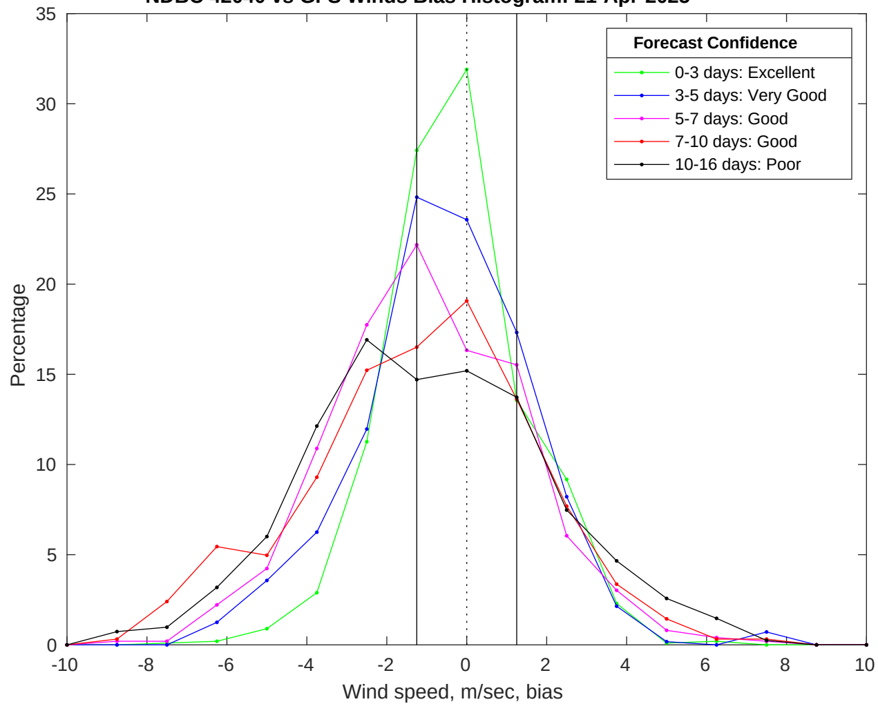
NDBC 42040 vs GFS Winds Bias Histogram: 21-Apr-2025
