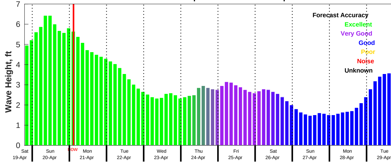
CMEMS Wave Forecast for NDBC 42040 from 19-Apr-2025 19:00:00 to 29-Apr-2025 19:00:00
