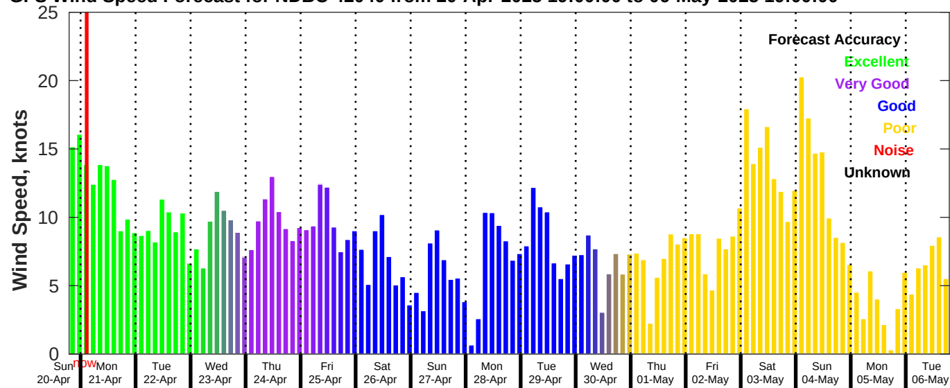
GFS Wind Speed Forecast for NDBC 42040 from 20-Apr-2025 19:00:00 to 06-May-2025 19:00:00
