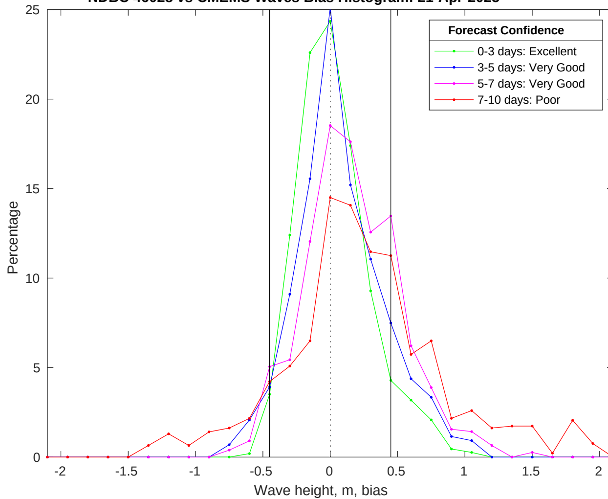
NDBC 46028 vs CMEMS Waves Bias Histogram: 21-Apr-2025
