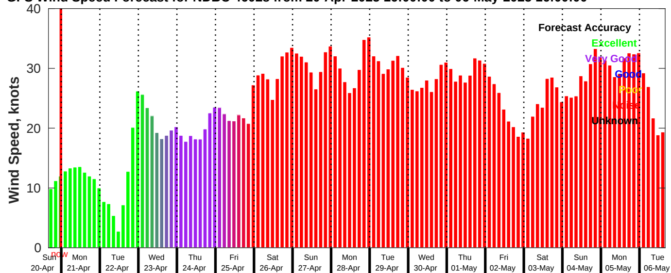
GFS Wind Speed Forecast for NDBC 46028 from 20-Apr-2025 16:00:00 to 06-May-2025 16:00:00
