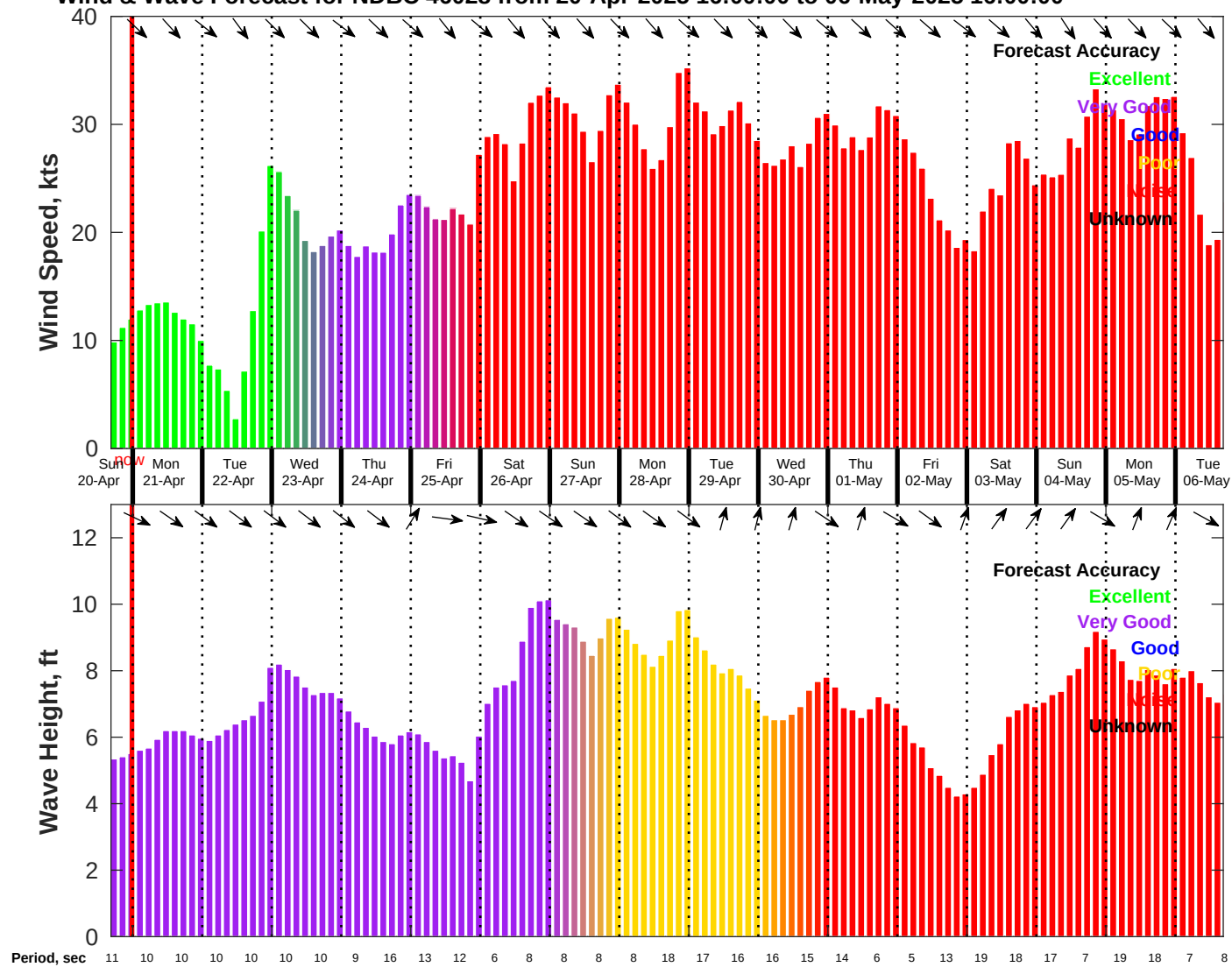
Wind & Wave Forecast for NDBC 46028 from 20-Apr-2025 16:00:00 to 06-May-2025 16:00:00
