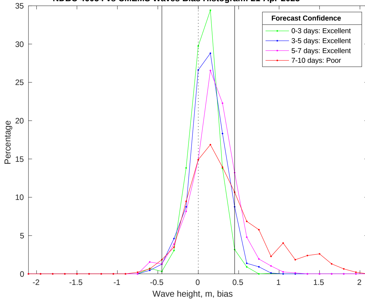
NDBC 46054 vs CMEMS Waves Bias Histogram: 21-Apr-2025
