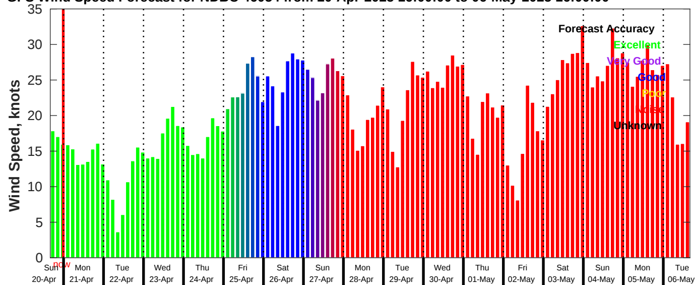
GFS Wind Speed Forecast for NDBC 46054 from 20-Apr-2025 16:00:00 to 06-May-2025 16:00:00
