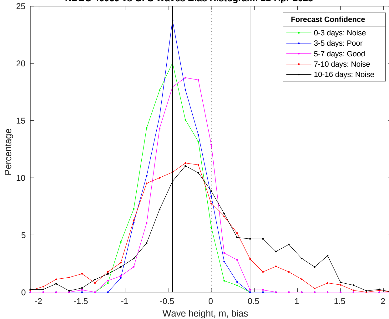
NDBC 46069 vs GFS Waves Bias Histogram: 21-Apr-2025
