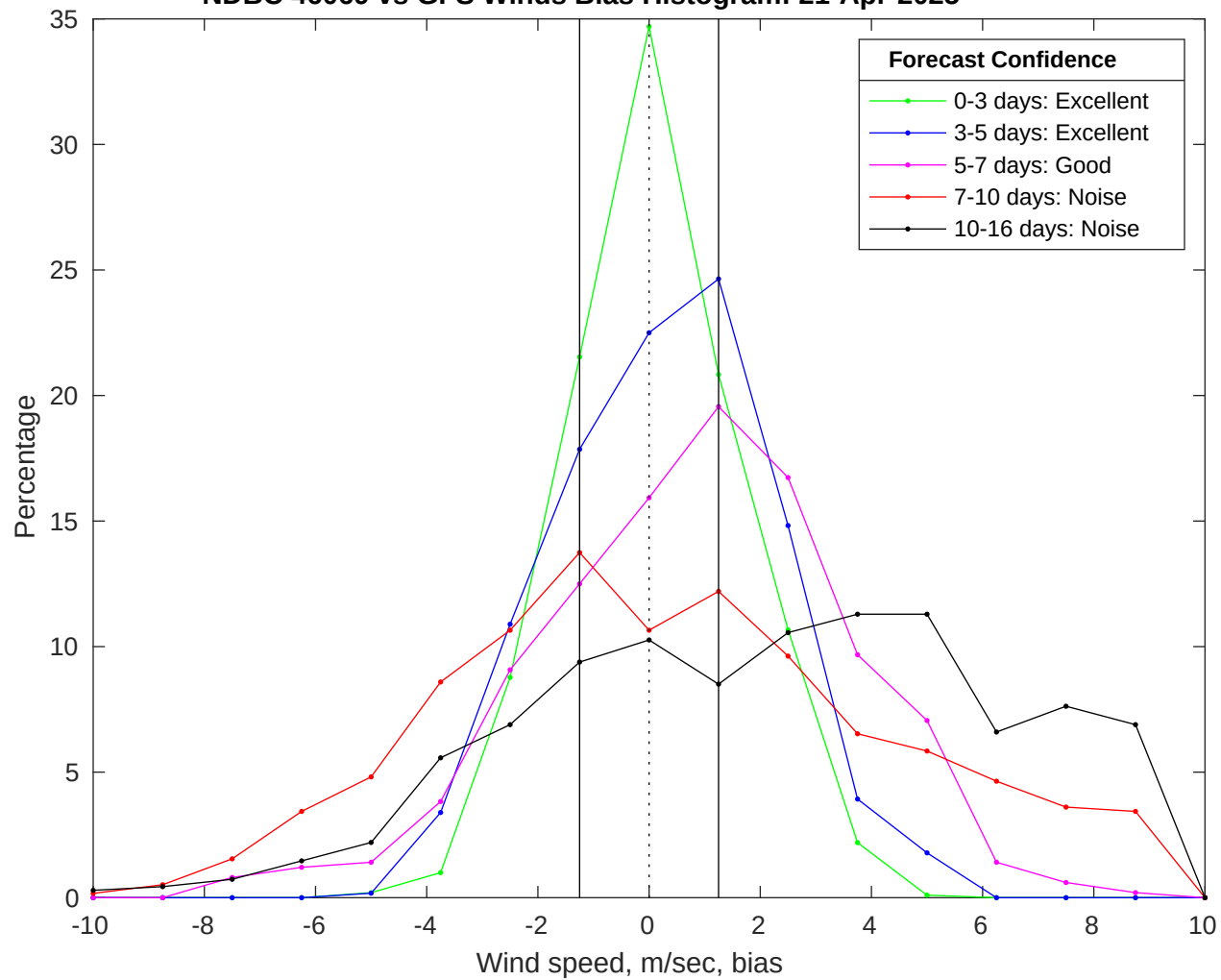
NDBC 46069 vs GFS Winds Bias Histogram: 21-Apr-2025
