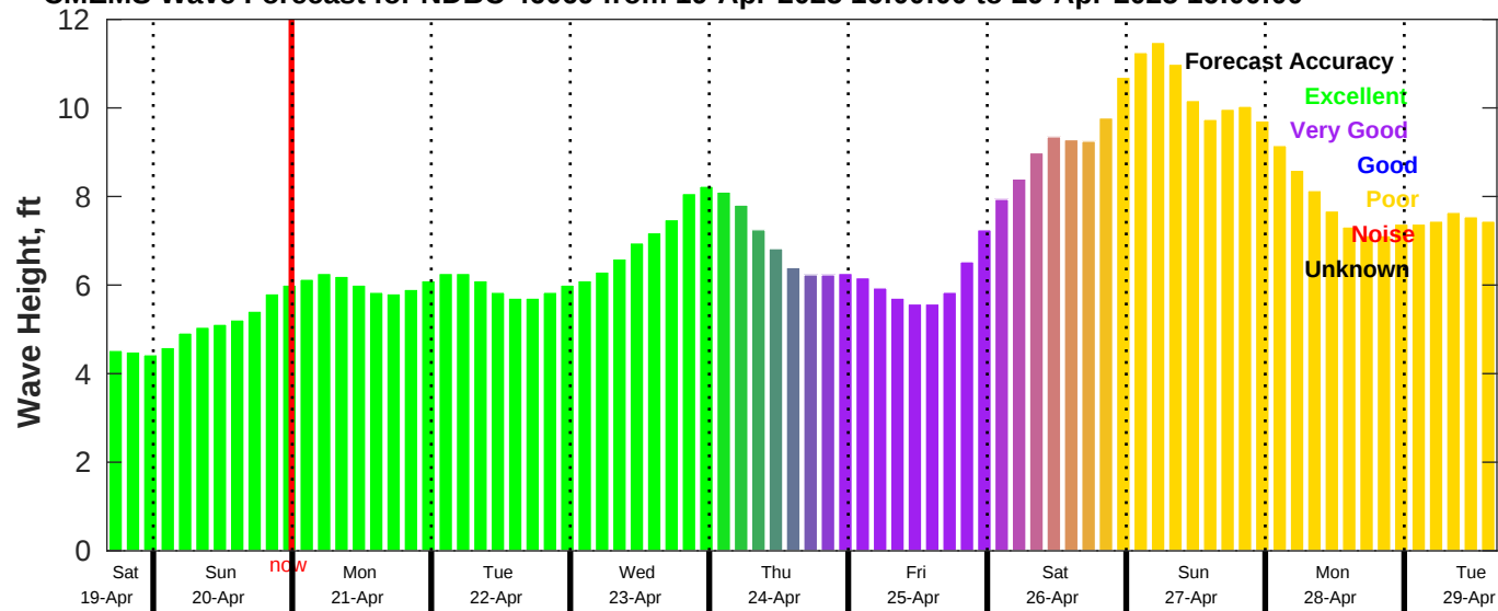
CMEMS Wave Forecast for NDBC 46069 from 19-Apr-2025 16:00:00 to 29-Apr-2025 16:00:00
