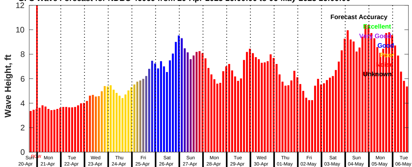
GFS Wave Forecast for NDBC 46069 from 20-Apr-2025 16:00:00 to 06-May-2025 16:00:00
