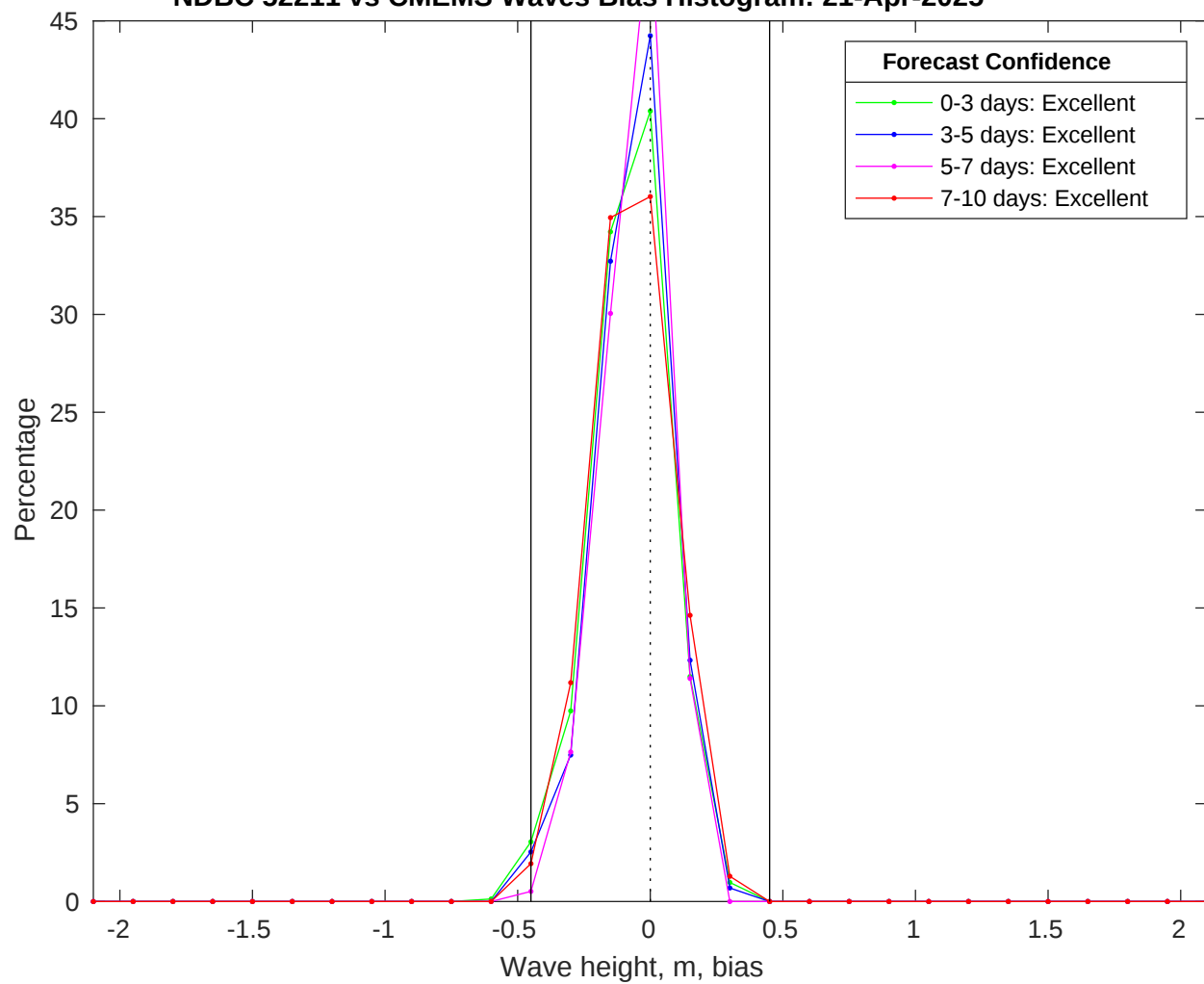
NDBC 52211 vs CMEMS Waves Bias Histogram: 21-Apr-2025
