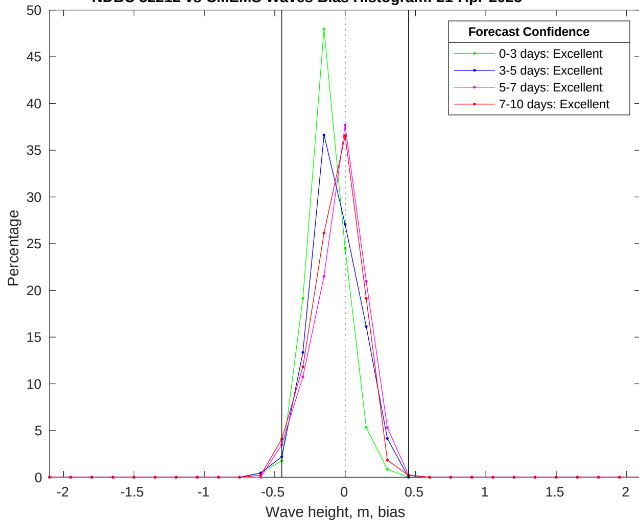
NDBC 52212 vs CMEMS Waves Bias Histogram: 21-Apr-2025
