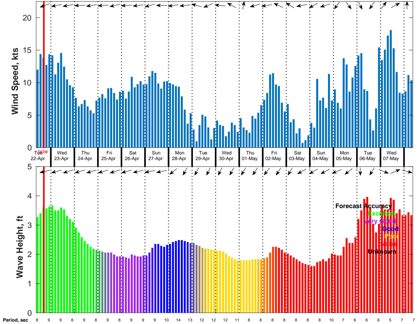
Wind & Wave Forecast for NDBC 52212 from 21-Apr-2025 09:00:00 to 07-May-2025 09:00:00
