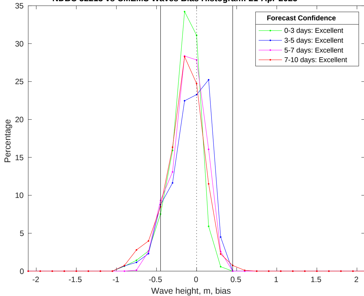
NDBC 52213 vs CMEMS Waves Bias Histogram: 21-Apr-2025
