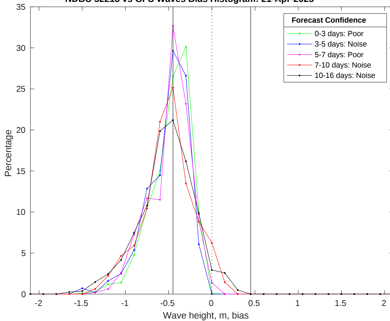
NDBC 52213 vs GFS Waves Bias Histogram: 21-Apr-2025
