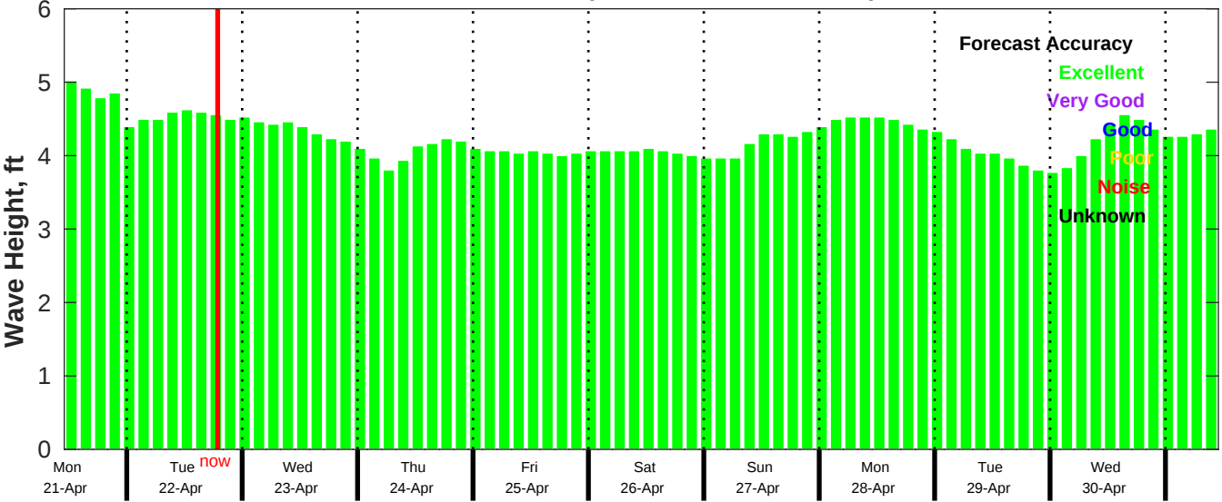
CMEMS Wave Forecast for NDBC 52213 from 20-Apr-2025 11:00:00 to 30-Apr-2025 11:00:00
