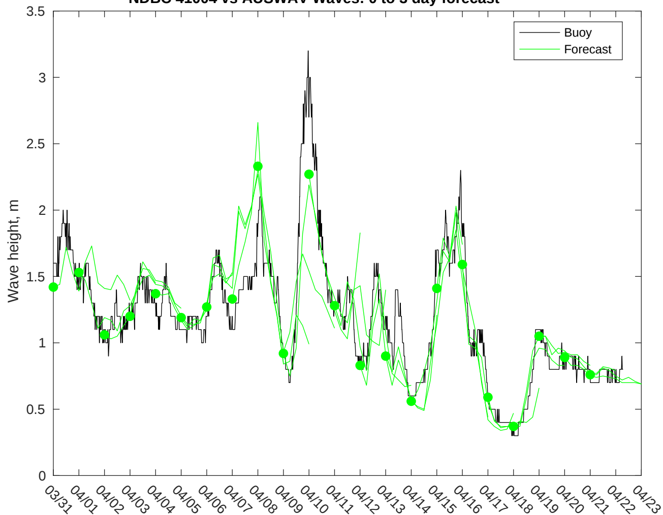
NDBC 41004 vs AUSWAV Waves: 0 to 3 day forecast
