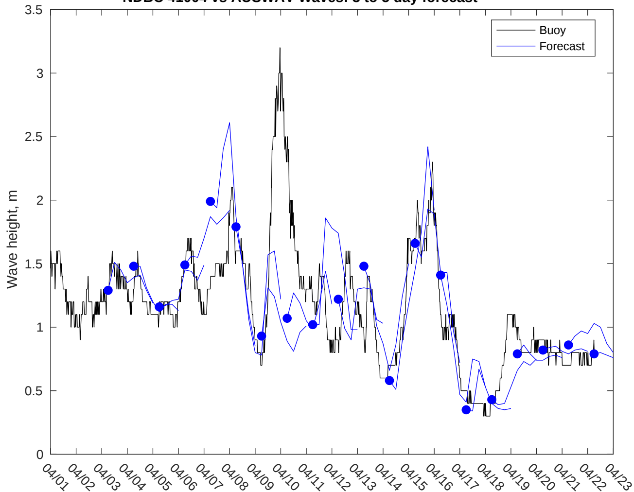
NDBC 41004 vs AUSWAV Waves: 3 to 5 day forecast
