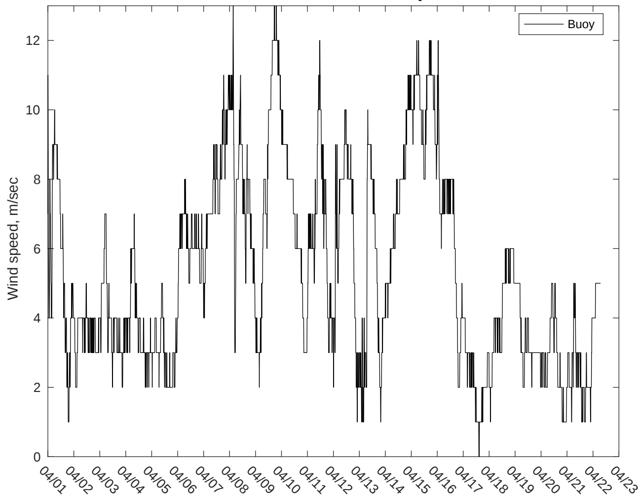
NDBC 41004 vs AUSWAV Winds: 10 to 16 day forecast
