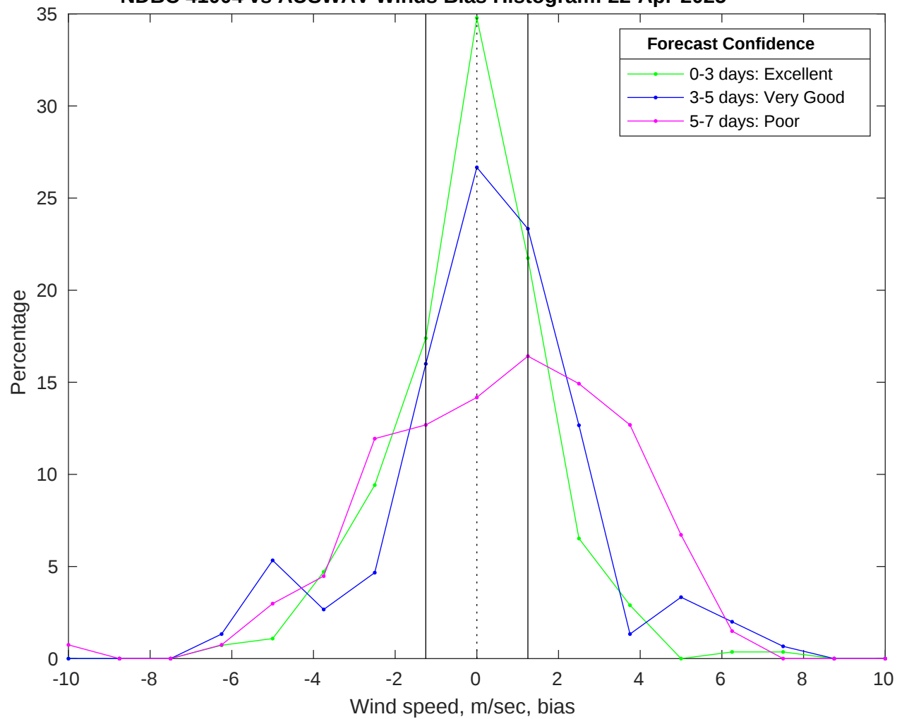
NDBC 41004 vs AUSWAV Winds Bias Histogram: 22-Apr-2025
