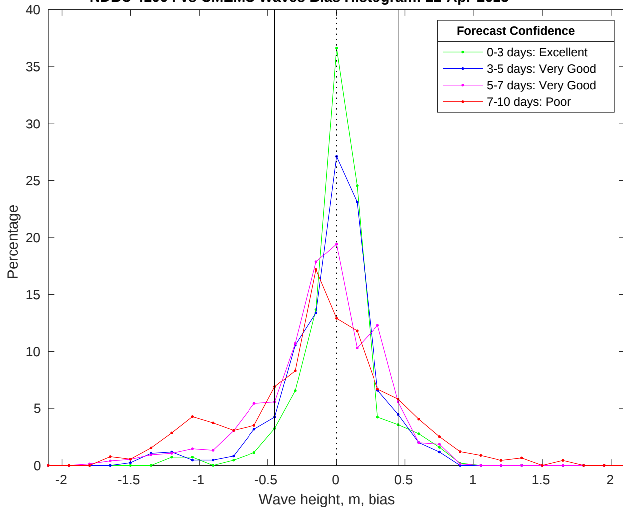
NDBC 41004 vs CMEMS Waves Bias Histogram: 22-Apr-2025
