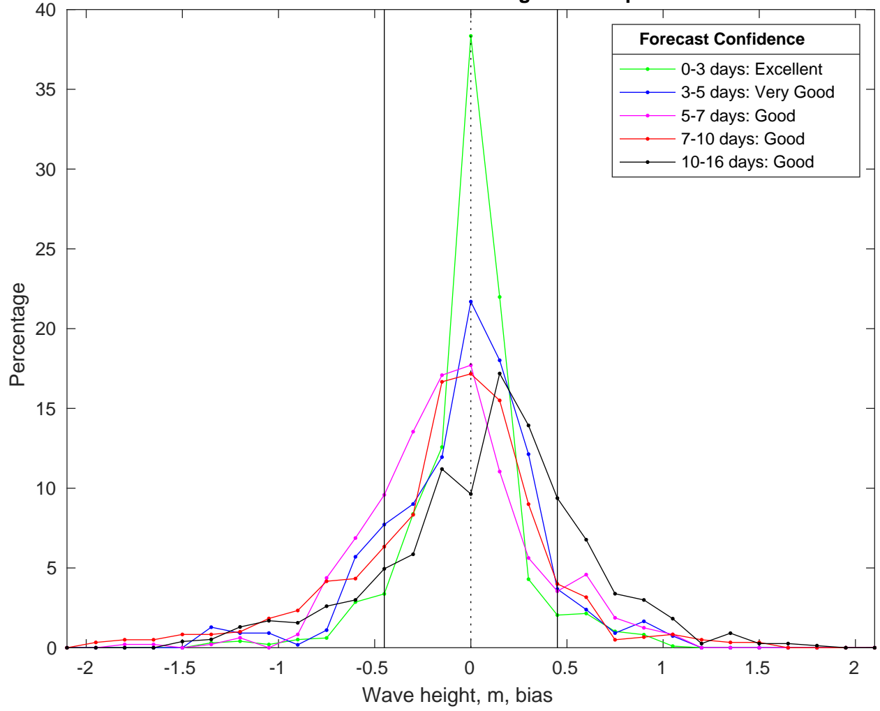
NDBC 41004 vs GFS Waves Bias Histogram: 22-Apr-2025
