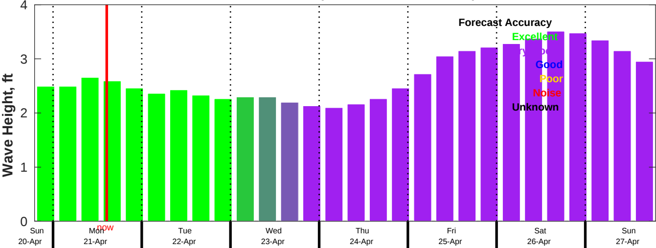
AUSWAV Wave Forecast for NDBC 41004 from 20-Apr-2025 19:00:00 to 27-Apr-2025 19:00:00
