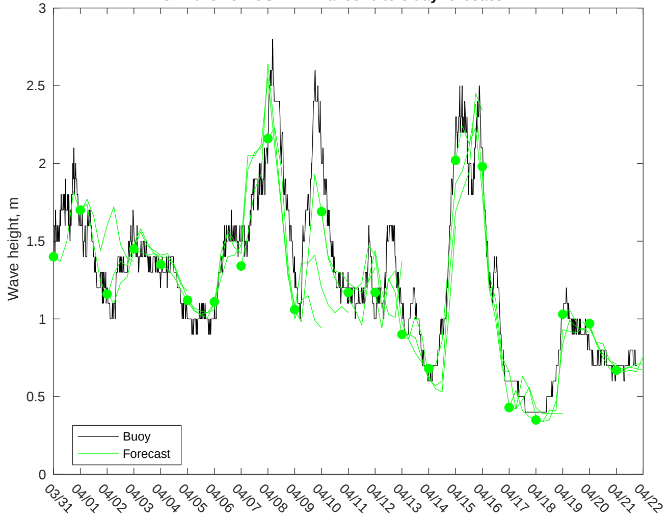
NDBC 41013 vs AUSWAV Waves: 0 to 3 day forecast
