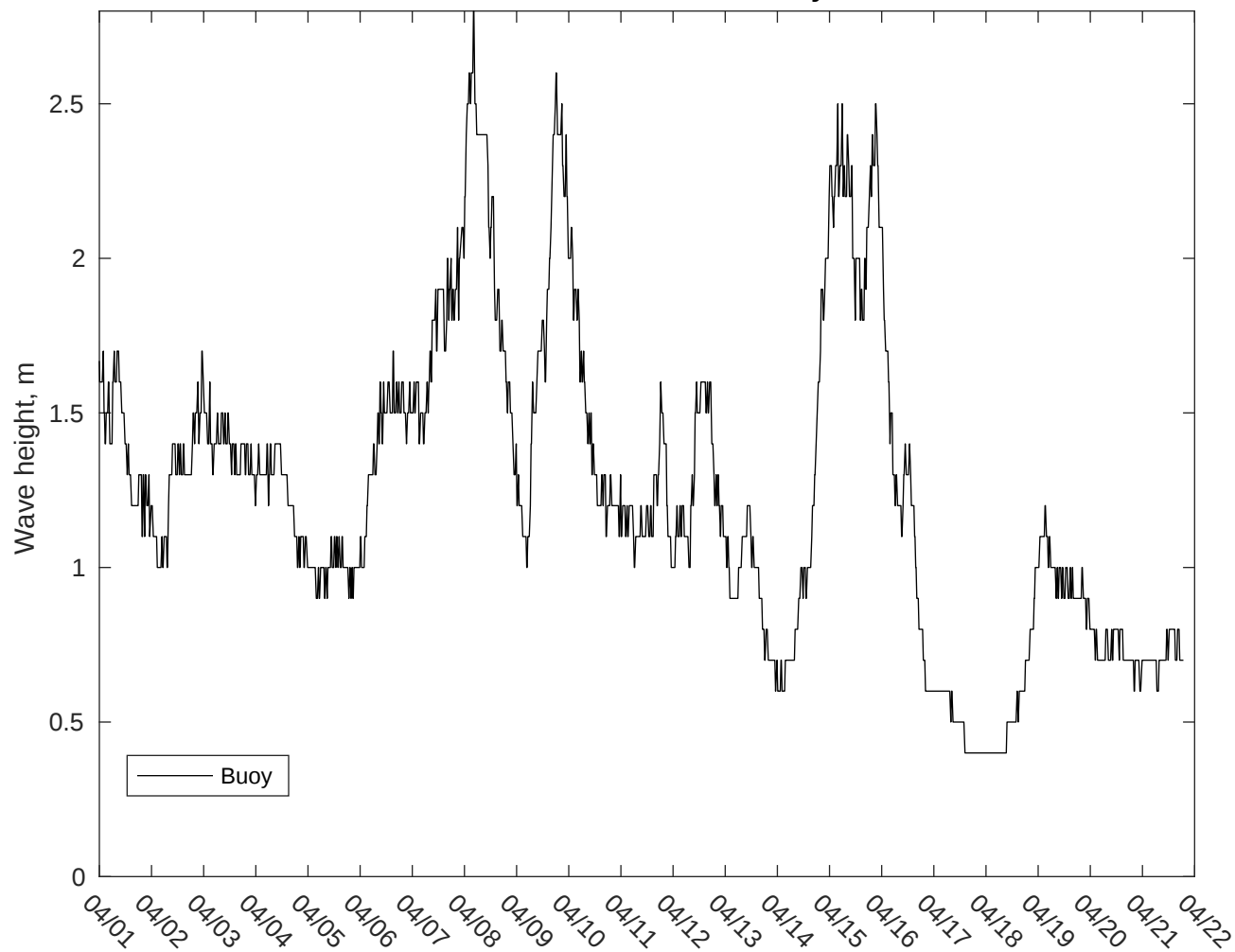
NDBC 41013 vs AUSWAV Waves: 10 to 16 day forecast
