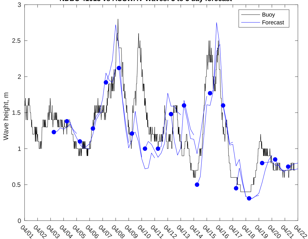
NDBC 41013 vs AUSWAV Waves: 3 to 5 day forecast
