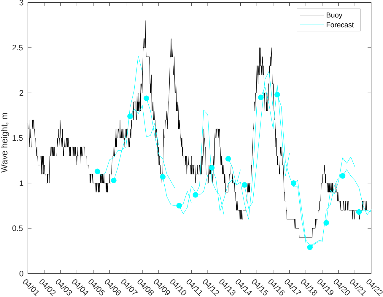
NDBC 41013 vs AUSWAV Waves: 5 to 7 day forecast
