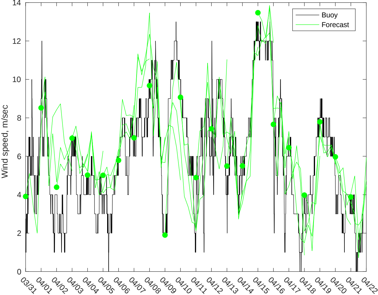
NDBC 41013 vs AUSWAV Winds: 0 to 3 day forecast
