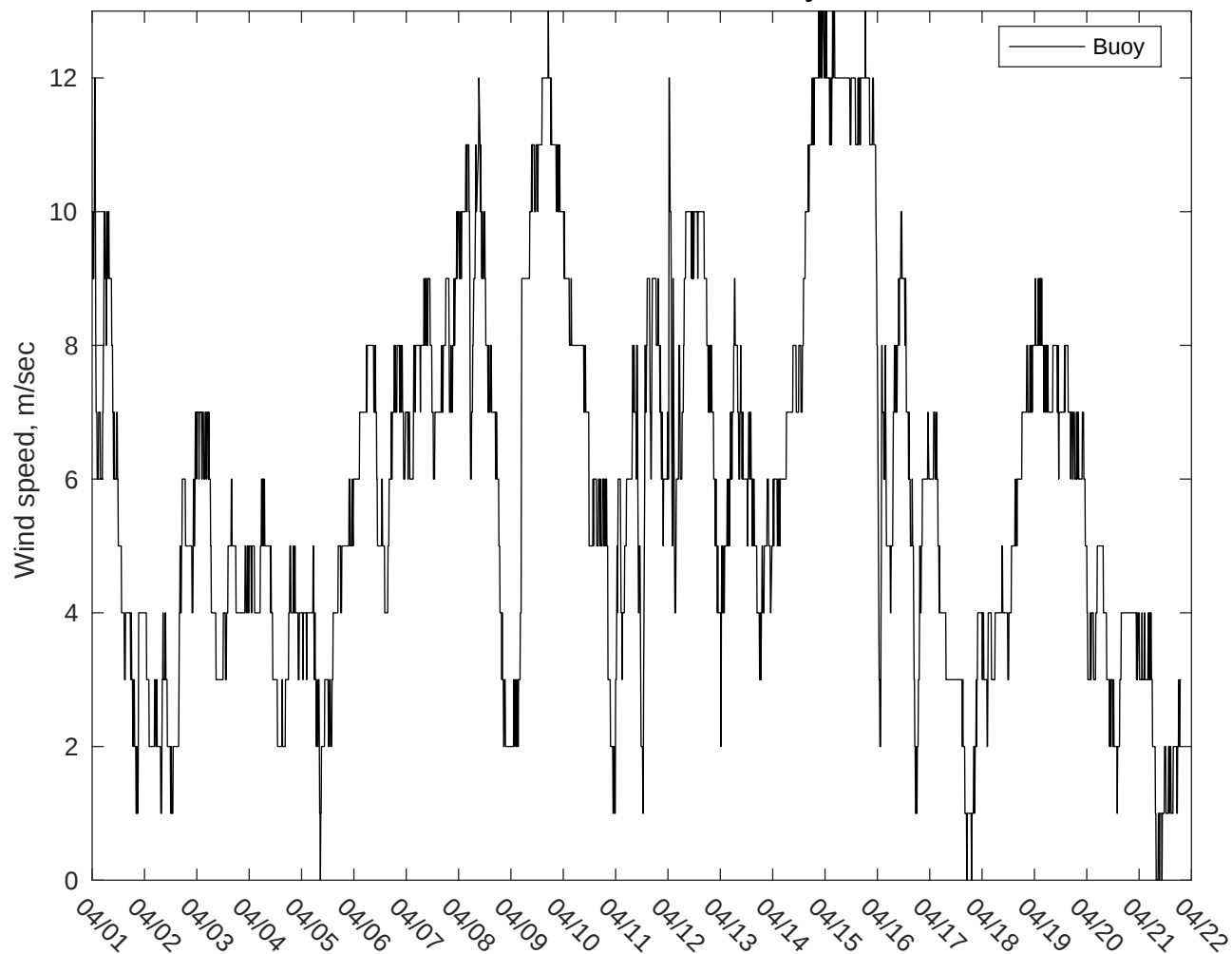
NDBC 41013 vs AUSWAV Winds: 10 to 16 day forecast
