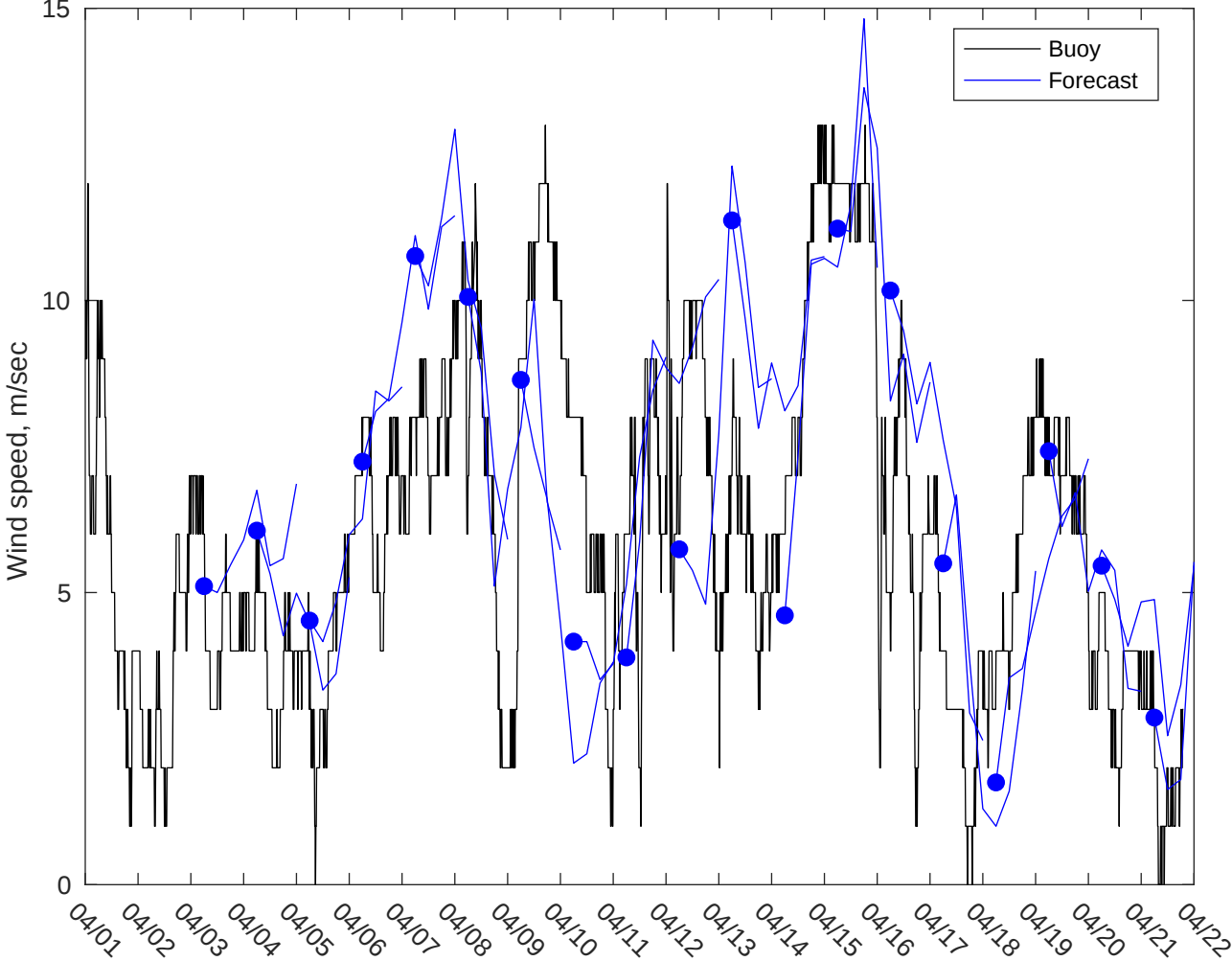
NDBC 41013 vs AUSWAV Winds: 3 to 5 day forecast
