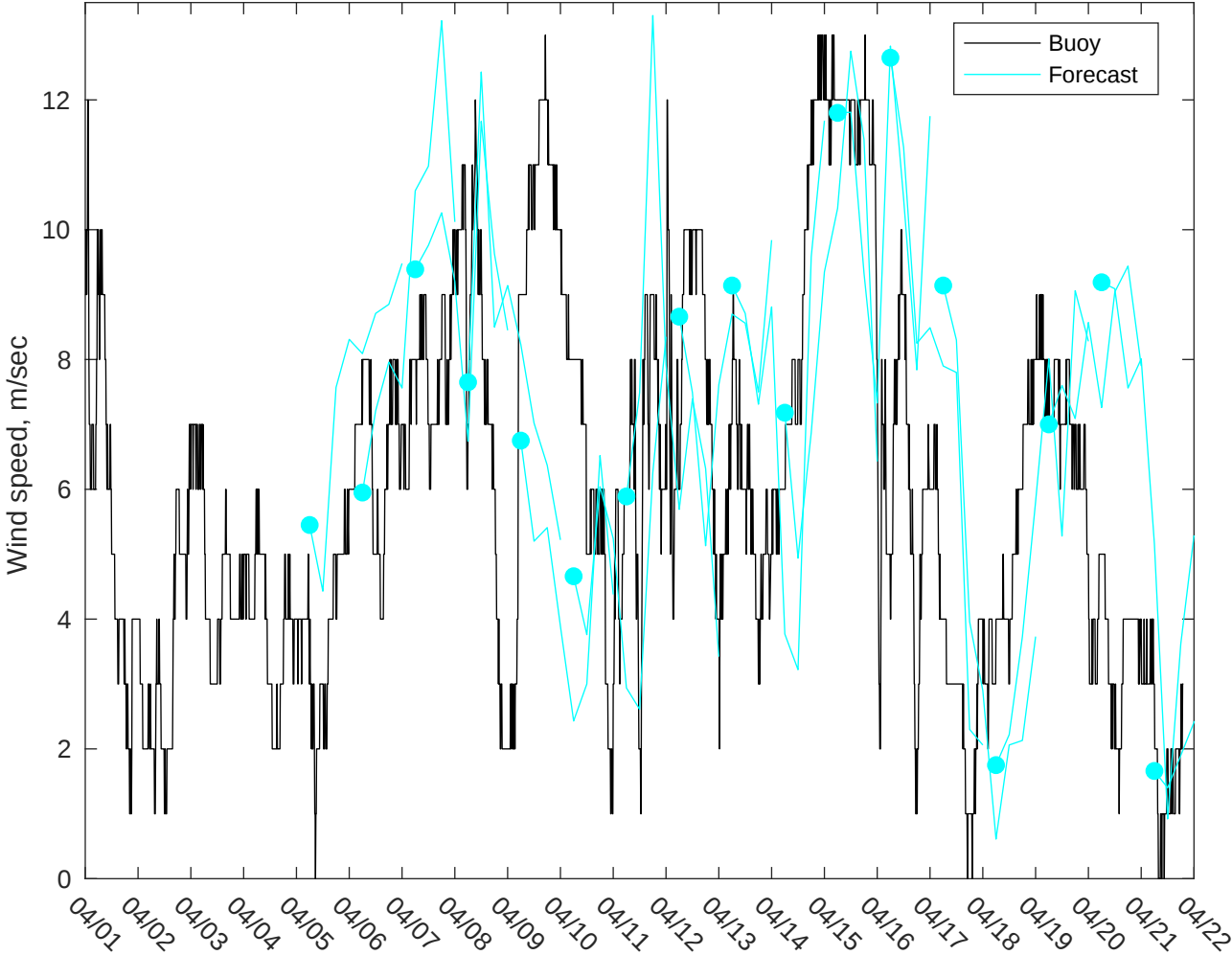
NDBC 41013 vs AUSWAV Winds: 5 to 7 day forecast
